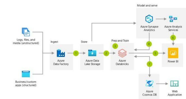
Figure.1: Accelerate ETL with Azure Databricks
